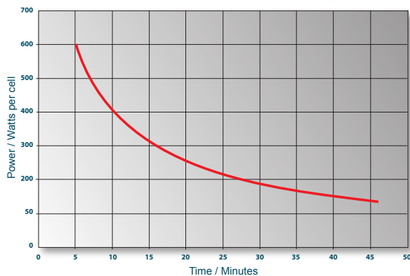
NSB12-330 Discharge Curve to 1.67 vpc
